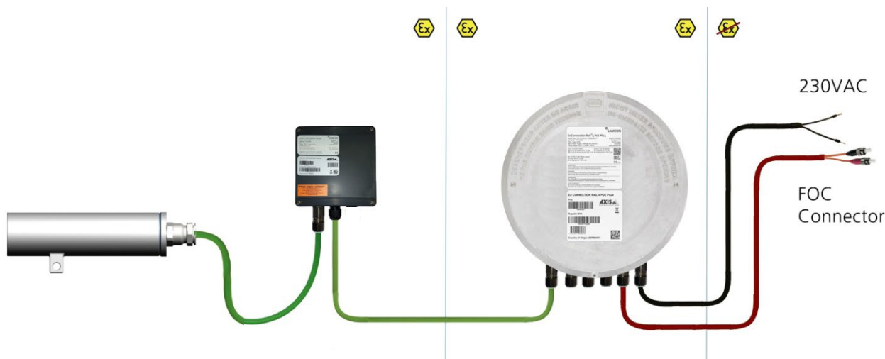
Bild 5-9 ExTB-2 -> ExConnection Rail
