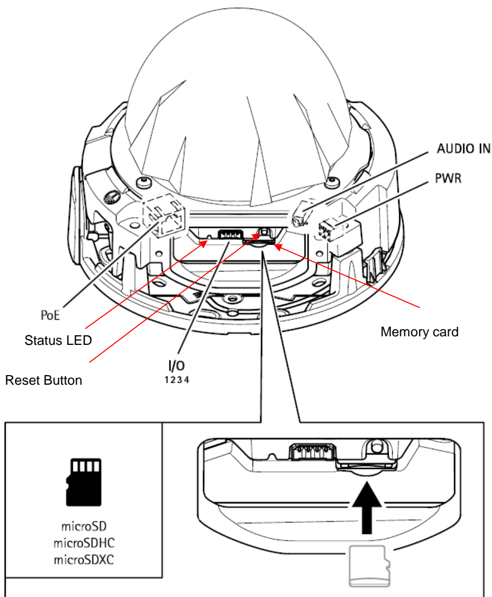
Figure 6-3 Reset Button / Memory Card
